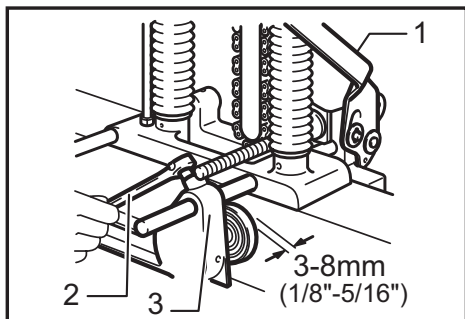
► 1. Lever (A) 2. Rear vise 3. Vise lever
