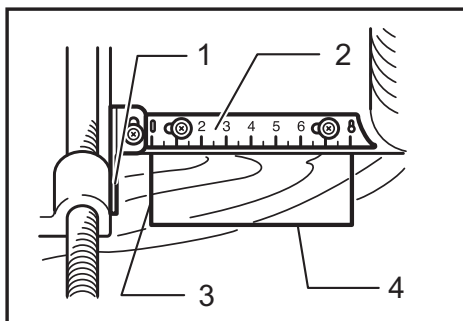
► 1. Indicator plate 2. Indication plate 3. Cutting line (A) 4. Cutting line (B)
